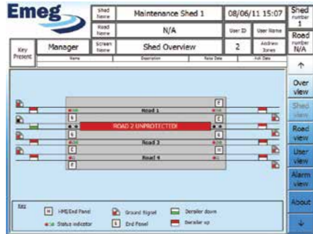
Typical screen image showing shed overview.
